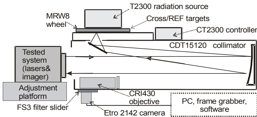
Fig. 2. Block diagram of the JALI boresight system
